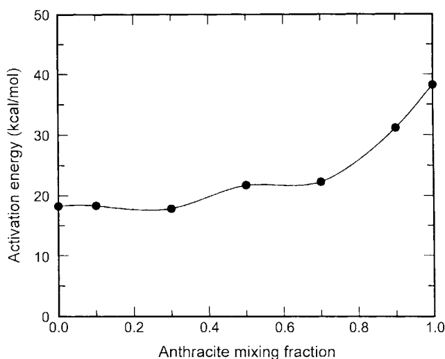
Fig. 3. Activation energy with anthracite mixing fraction.
